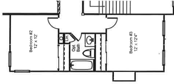
Newport III Optional Second Floor Bathroom Plan
